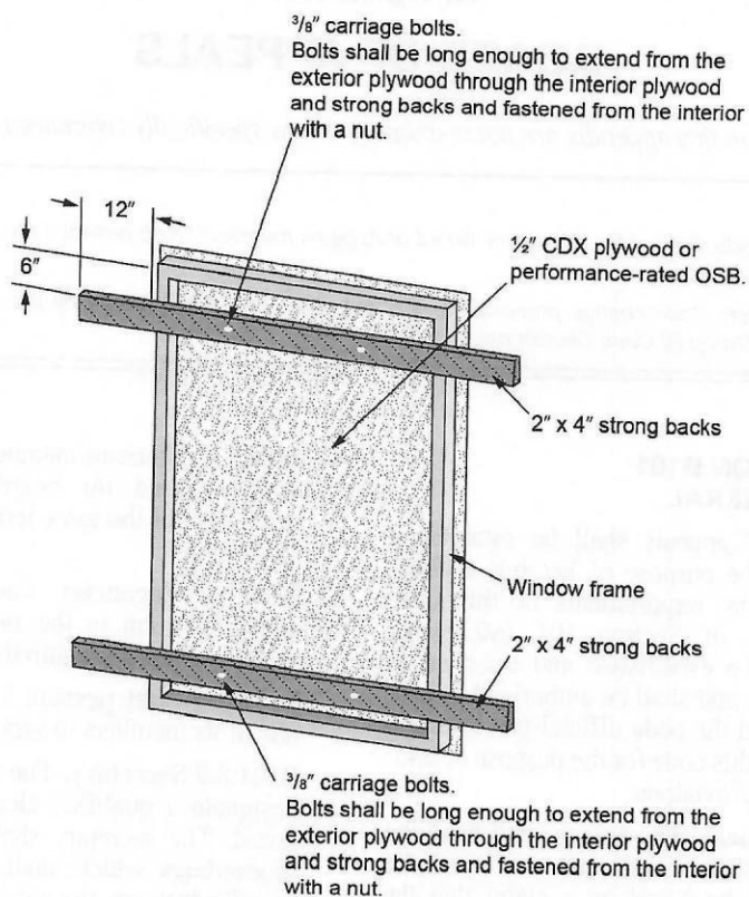
FIGURE A103.1(1) BOARDING OF DOOR OR WINDOW
